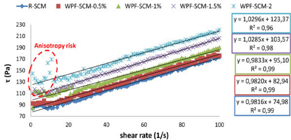
Fig. (7). Shear stress for WPF-SCM mixtures.
