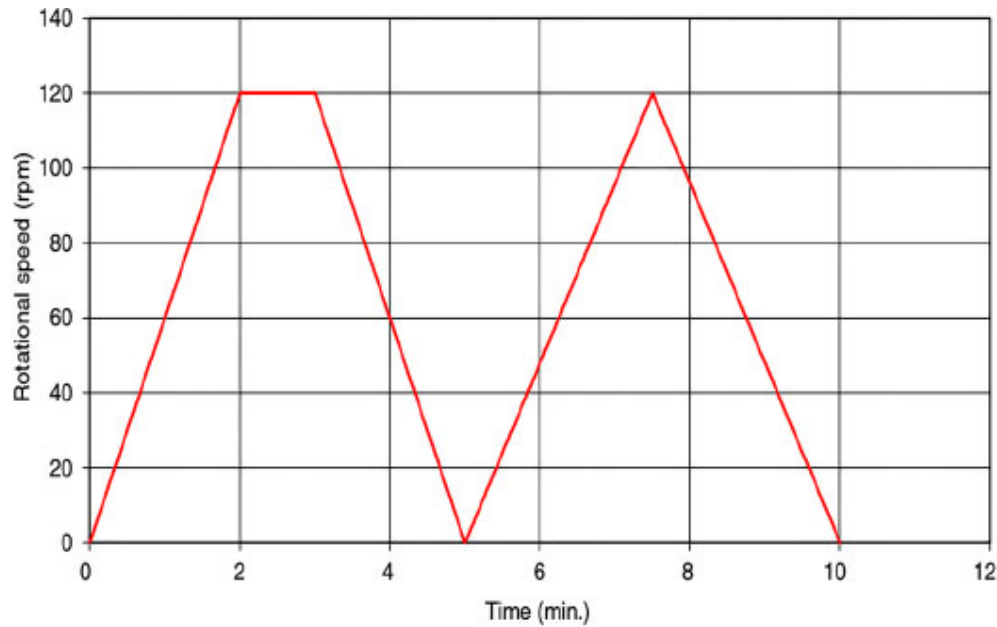
Fig. (3). Rotation speed monitored over the first 10 minutes [18].
