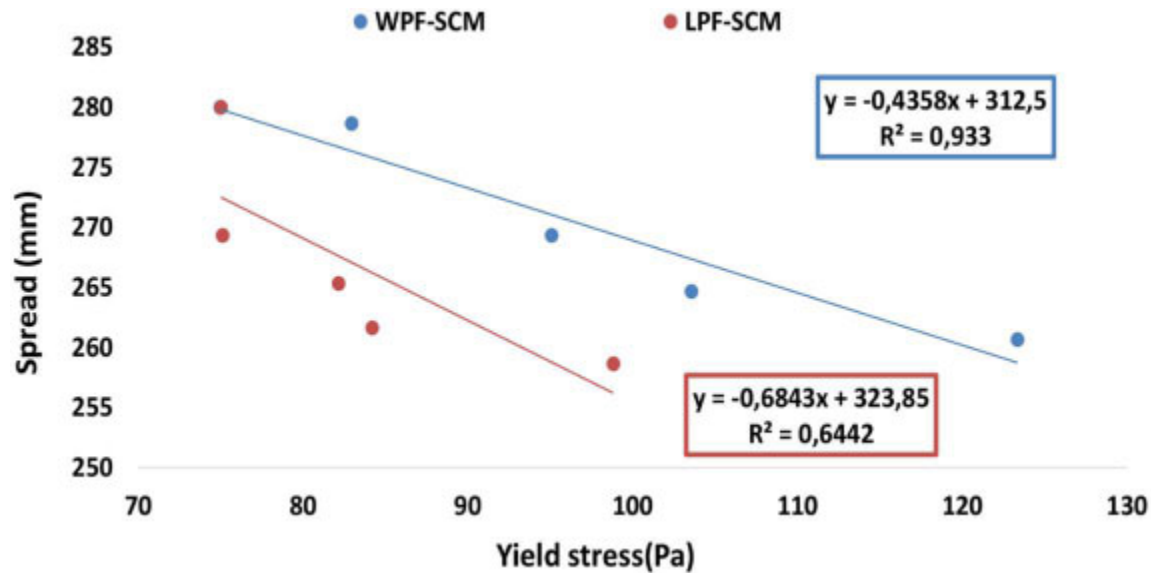
Fig. (12). Flow- yield stress relationship.
