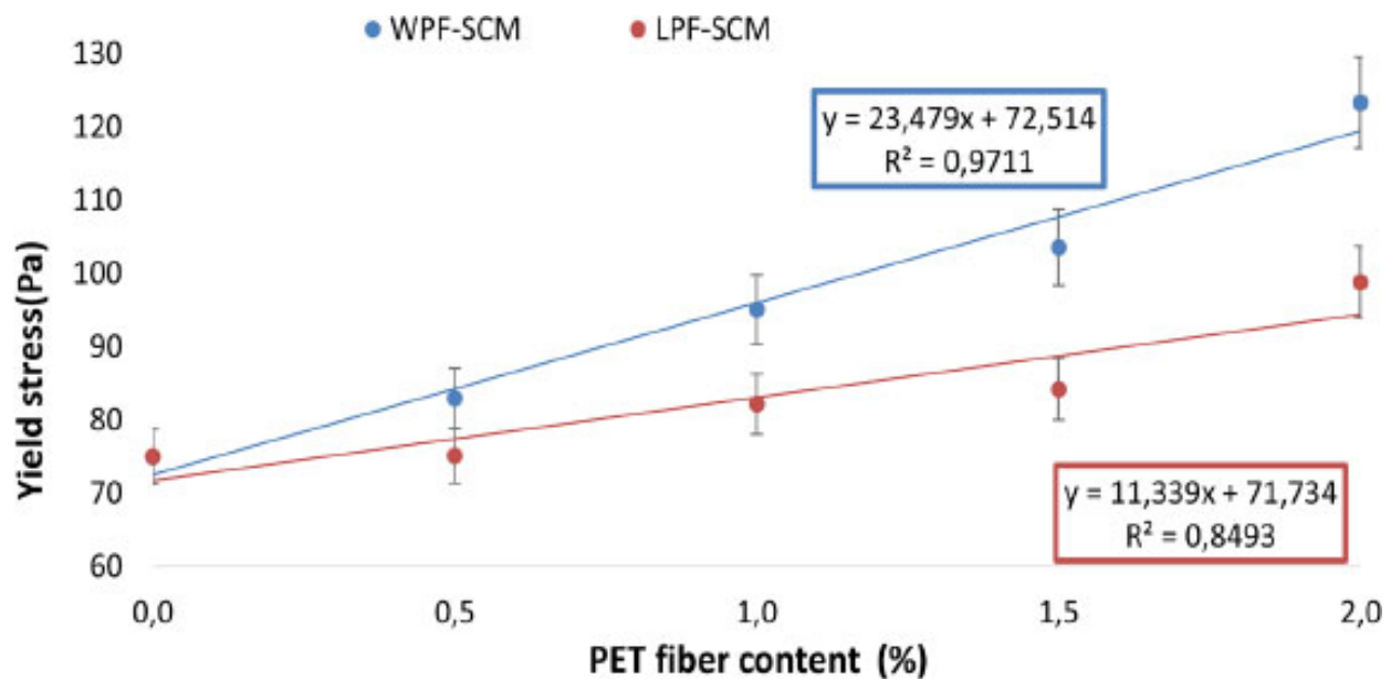
Fig. (9). Rheological behaviour of PF-SCM mixtures: Yield stress.
