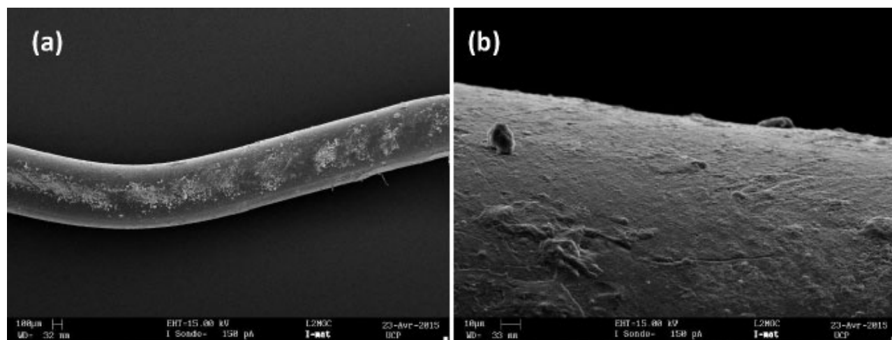
Fig. (10). SEM analysis of wavy PET fibres.
