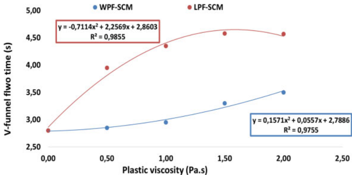
Fig. (13). Flow time- plastic viscosity relationship.
