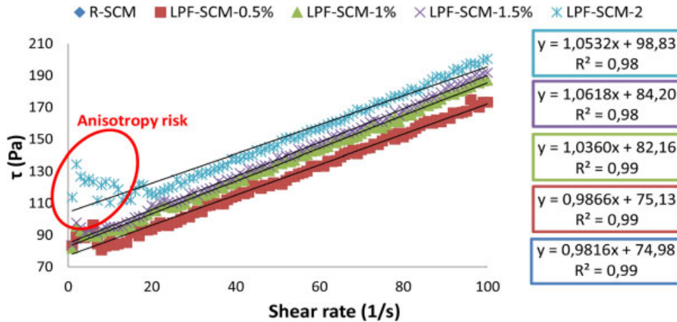
Fig. (6). Shear stress for LPF-SCM mixtures.
