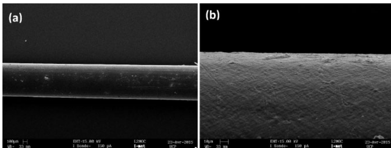
Fig. (11). SEM analysis of linear PET fibres.
