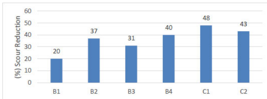
Fig. (10). Reduction percentage of relative scour depths at F_G 1.91.
