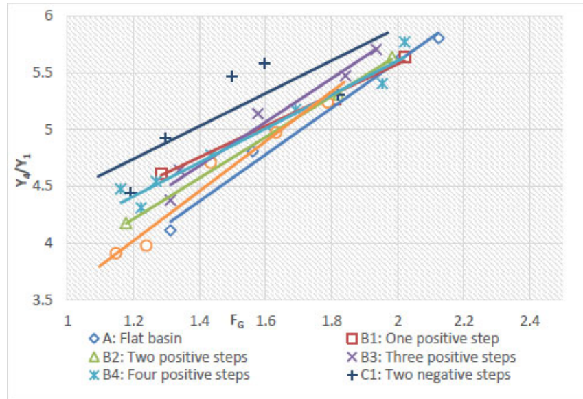
Fig. (11). Relationship between Relative Depth Ratio ( Y_4/Y_1 ) and Gate Froude Number ( F_g ) for Different Basin Configuration.
