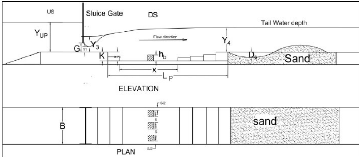
Fig. (1). Definition sketches for the experimental model.
