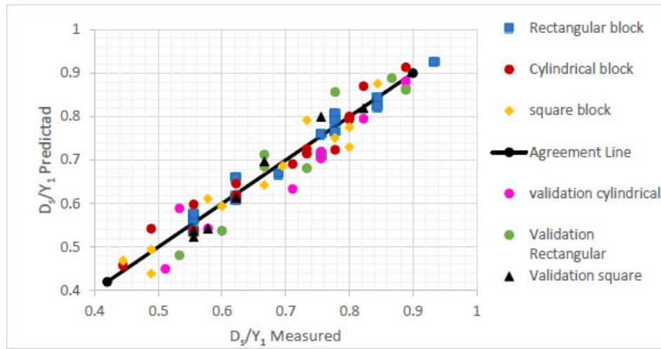
Fig. (20). Relation between the measured and predicted data for different shapes of baffle blocks.
