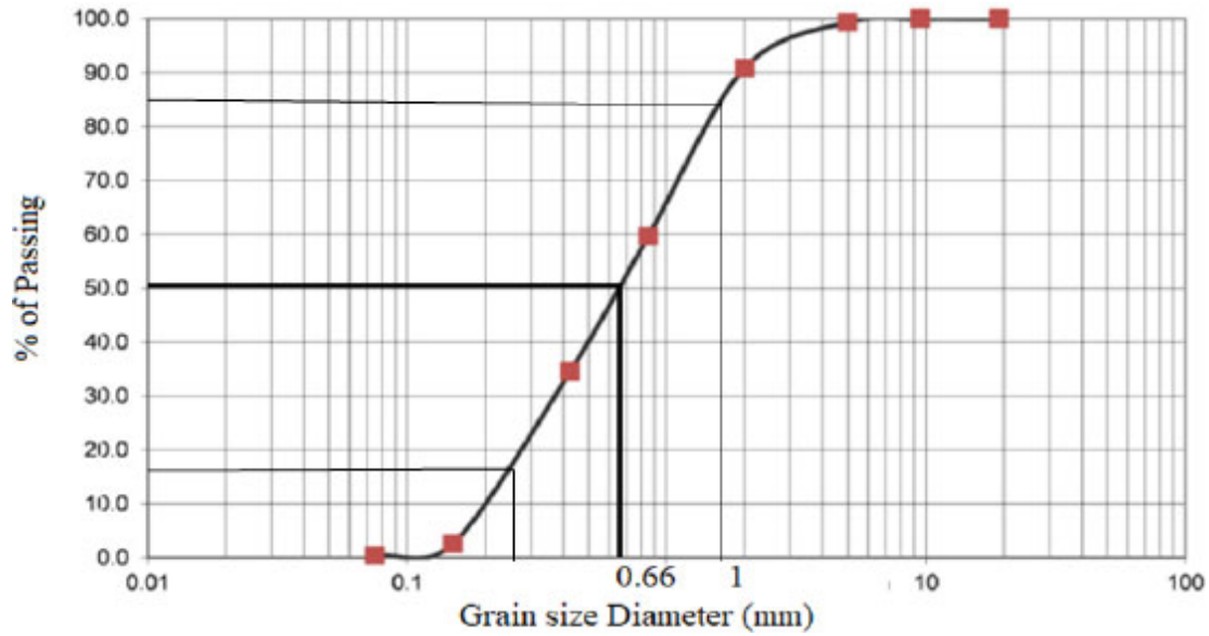
Fig. (5). Particle size distribution for particle bed.
