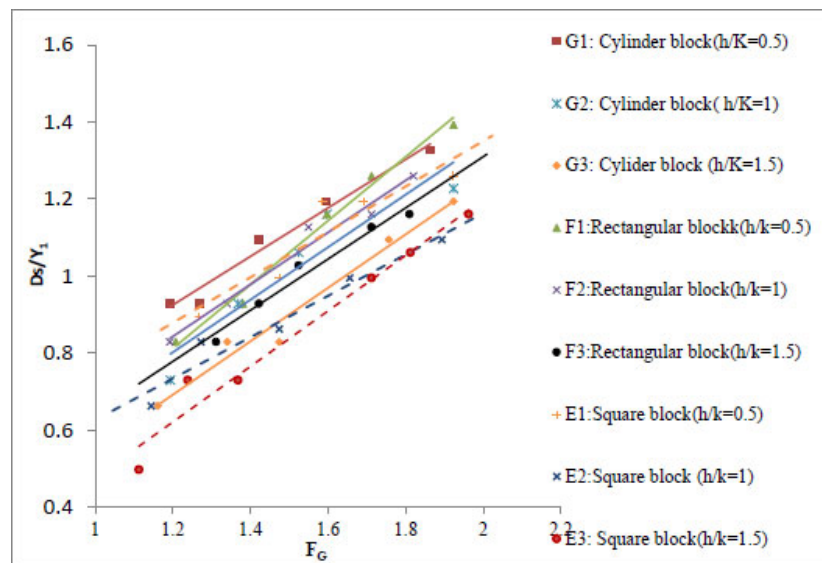
Fig. (14). Effects of the shapes and relative height of baffle blocks on the relative scour depth with the gate Froude number ( F_G ).
