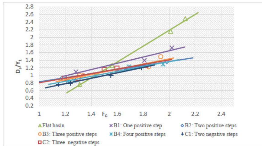
Fig. (9). Effects of different shapes, B, C, and the flat basin model A, on maximum scour depth.
