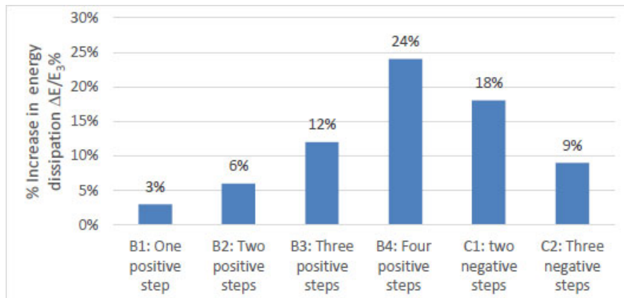
Fig. (8). Percentage increase in relative energy dissipation compared to flat basin at F_g 1.91.
