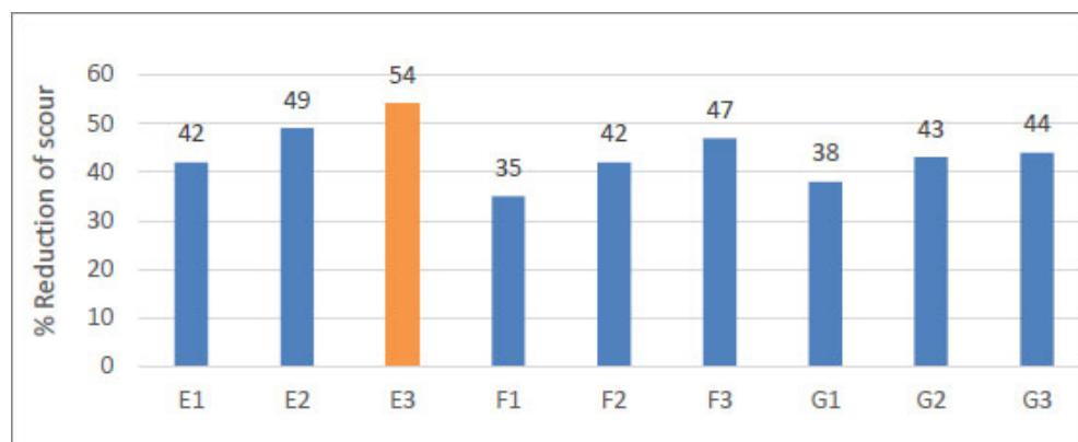
Fig. (18). Reduction percentage of relative scour depths at F_G = 1.91 .
