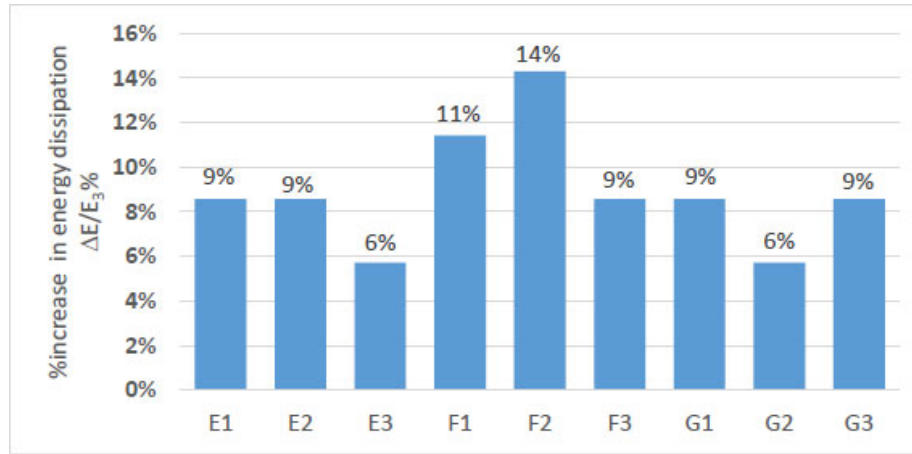
Fig. (19). Percentage increase in relative energy dissipation compared to flat basin at F_G 1.91.
