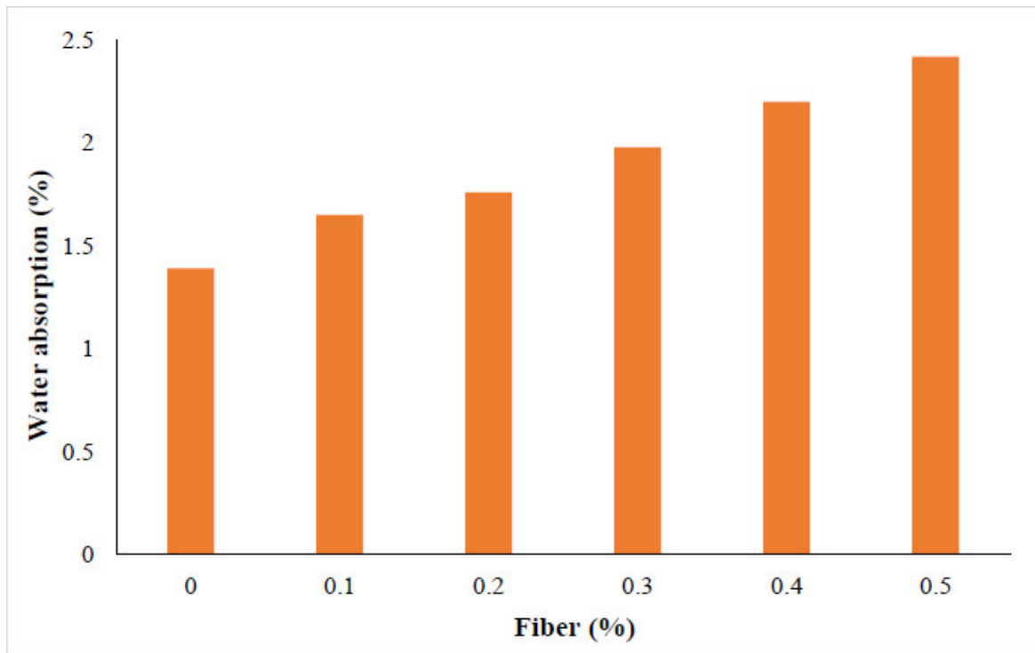
Fig. (3). Variation of water absorption test results.
